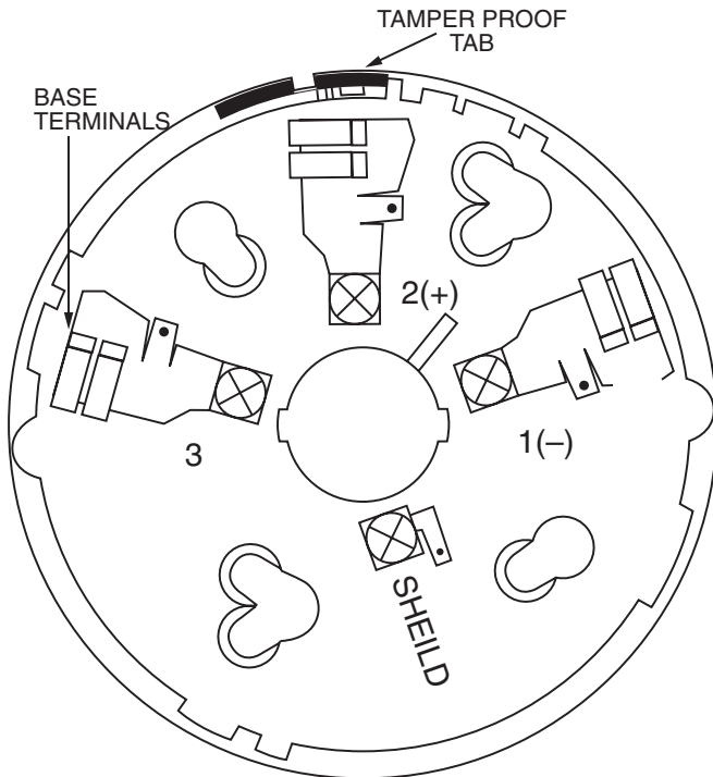
FIGURE 1. TERMINAL LAYOUT:
