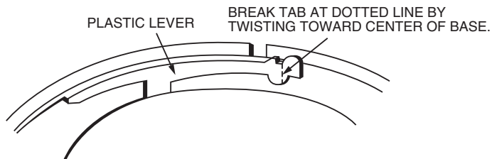
FIGURE 3A. ACTIVATING TAMPERPROOF FEATURE:
