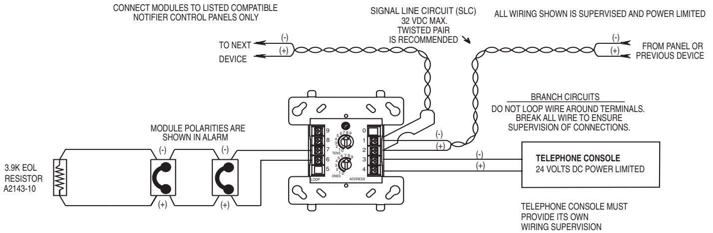
Figure 3. Typical circuit configuration, NFPA Style Y, Class B style wiring:
