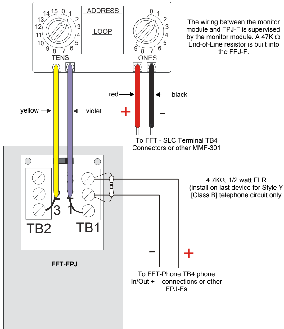
Figure 2.5 ECC-FFT Connections
