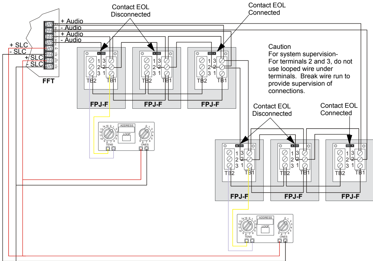
Figure 2.14 Multi-Phone Jack Audio Circuit in Class A
