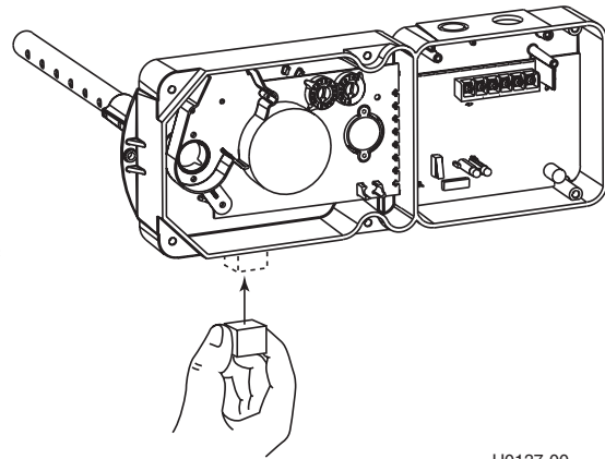
Figure 12. Testing detector alarm:
