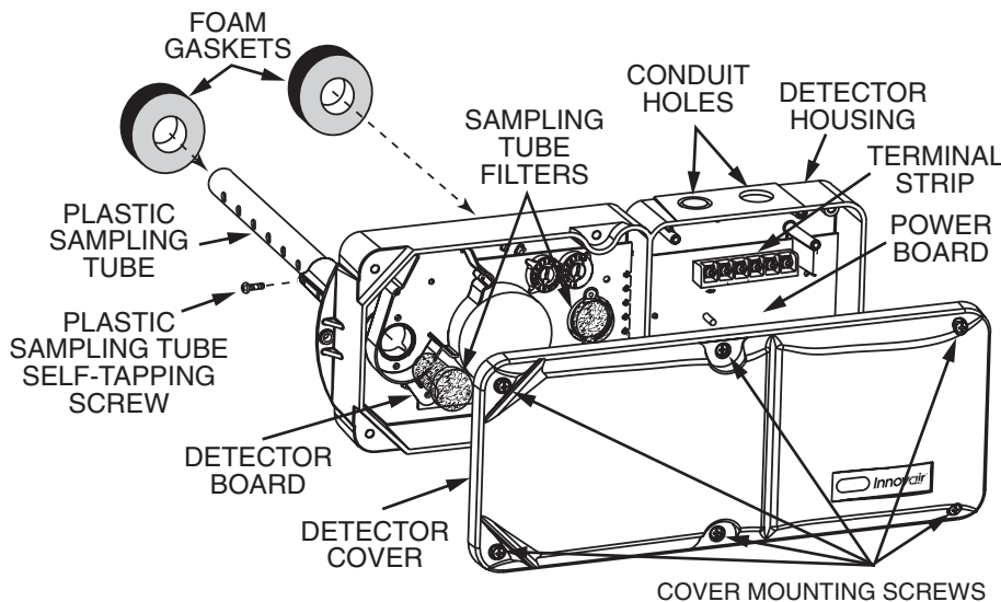
Figure 1: Exploded View Of Duct Smoke Detector Components
