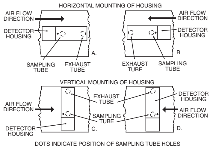
Figure 5. Tube mounting configurations with varying air flow direction:
