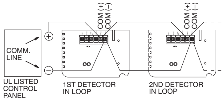
Figure 9. Wiring Diagram for D350PL Duct Smoke Detector using a UL listed control panel
