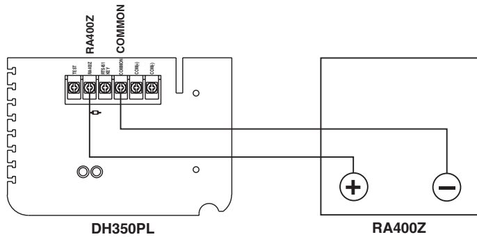
Figure 10. Wiring Diagram for D350PL Duct Detector with optional RA400Z
