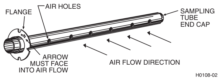
Figure 4. Air duct detector sampling tube:
