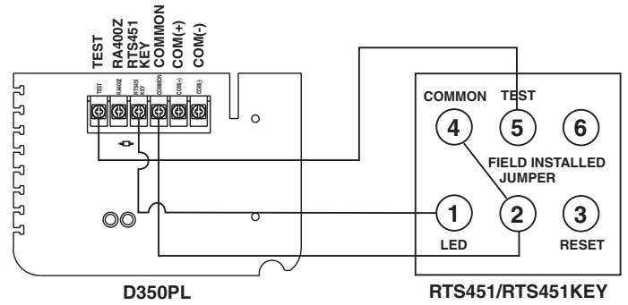
Figure 11. System Wiring Diagram for D350PL Duct Smoke Detector with RTS451/RTS451KEY
