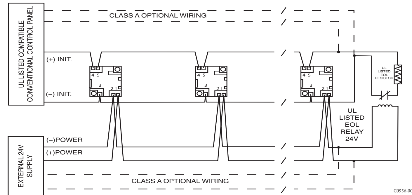
Figure 3. Typical wiring layout:
