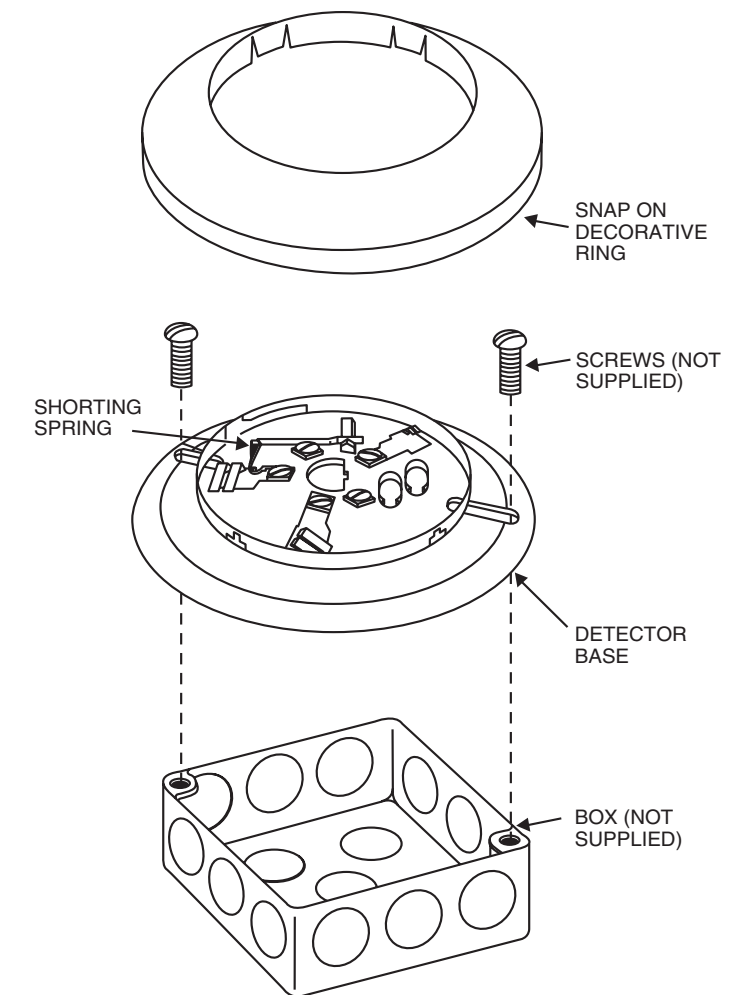
Figure 4. Mounting to an electrical box:
